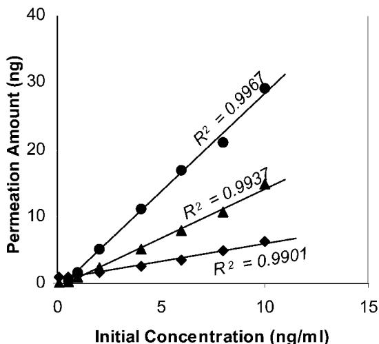
Fig. 2. Predicted linear relationship of permeation amount vs. initial concentrations. The scattered points were experimental values for terrazole ( \blacklozenge ), dacthal ( \bullet ), and chlorobenzilate ( \blacktriangle ). The solid lines were their corresponding linear regressions. The membrane-coated fiber was 100 \mu\text{m} PDMS, the initial concentrations of the donor solutions were from 0.1 to 10 ng/ml (each individual component), and the permeation time and stirring speed were kept as constants at 12 min and 400 rpm, respectively.
