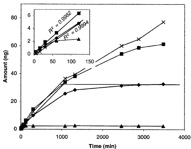
Fig. 3. MCF permeation profiles. The profiles of endosulfan sulfate ( \blacktriangle ), aldrin ( \blacklozenge ), tr-chlordane ( \blacksquare ), and p,p-DDT ( \times ) were measured by 100- \mu\text{m} PDMS MCFs in donor solutions of 75 ml 1.00 ng/ml (individual component). The insert was an expansion of the initial period of time.
